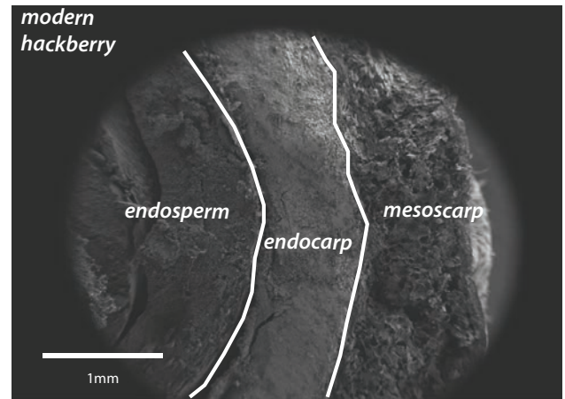
Figure 3. Scanning electron microscope image of the three distinct layers of a modern hackberry seed: (1) inner fruit or endosperm composed of partially mineralized spherical organic bodies, (2) endocarp consisting principally of aragonite and calcite, and (3) outer fruit or mesocarp with a framework of organic matter and some calcite crystals.
