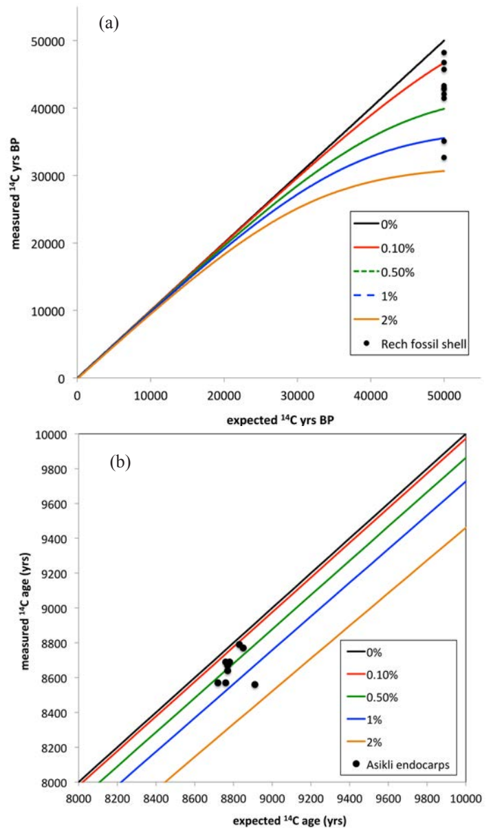
Figure 8. The effects on ^{14}\text{C} ages of variable (shown by lines 0.1 to 2%) modern contamination, compared to (a) fossil ( \geq 50 ka) shell reported on by Rech et al. (2011), and to (b) hackberry endocarps from Asıklı. Carbonate from both fossil shell and hackberries display subtle but measurable 0.1–2% contamination by modern carbon.
